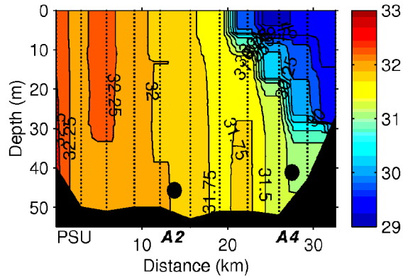
Figure 3. July 2003 CTD salinity section across the eastern channel of the Bering Strait from the Diomedede islands (left) to Alaska (right). Black dots indicate moored instrument locations. Note the fresh (warm) ACC on the Alaskan coast.
