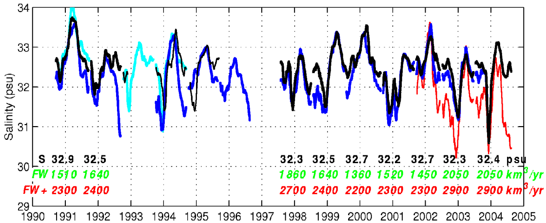
Figure 2. Thirty-day running mean of hourly time-series of salinity 9 m above bottom at sites A1 (western channel, cyan), A2 (eastern channel, blue), A3 (north of Bering Strait, black), and A4 (the Alaskan Coastal Current, red). Not all moorings are deployed each year. Between summer 1992 and summer 1995, A3' (thin black line) was deployed instead of A3 (see Figure 1). Record mean (i.e., ~ annual mean from summer to summer) salinities (S, black) (errors ~ 0.2 psu) and freshwater transports (errors ~ 300 km 3 /yr) are estimated from A3 records, assuming no stratification in velocity or density (FW, green) and with the correction of 800 km 3 /yr (FW+, red).
