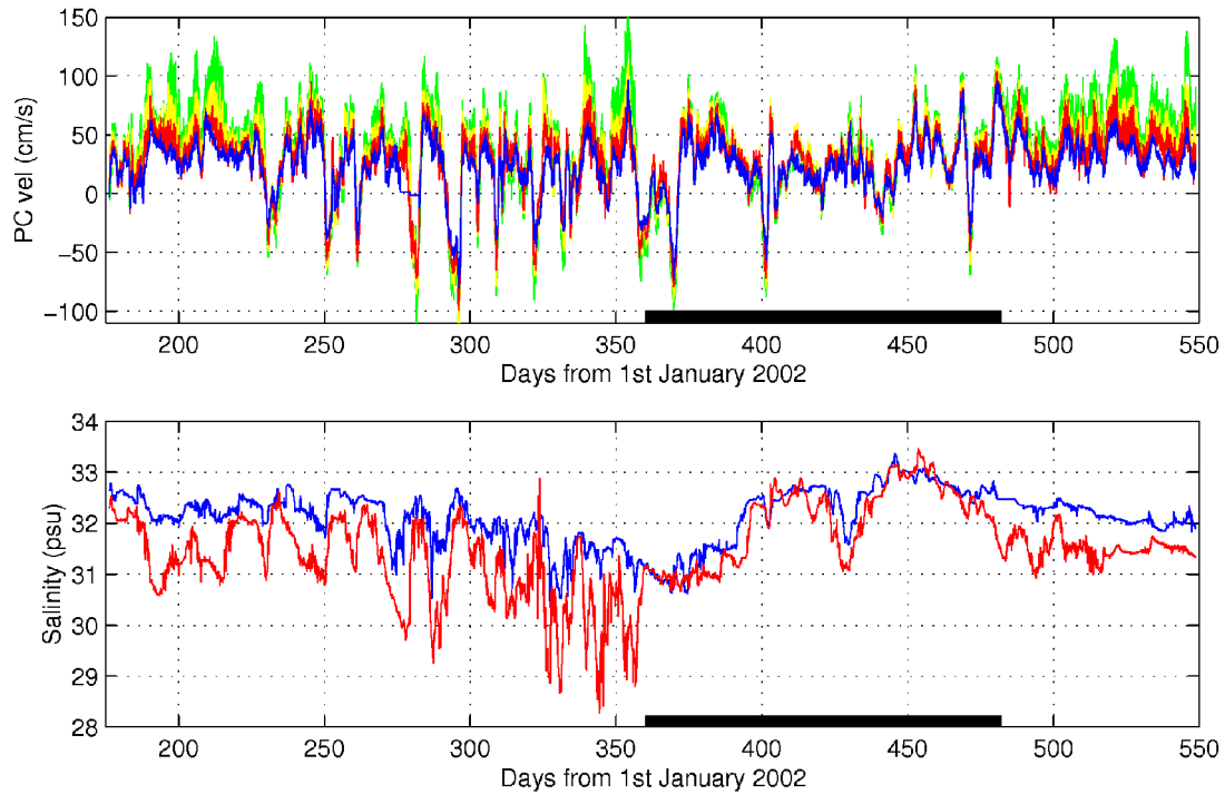
Figure 4. Hourly time-series data from A2 and A4 for July 2002 to 2003. (a) Principal component of velocity ( \sim northward velocity) at A2 (47 m, blue) and A4 (34 m, red; 24 m, yellow; and 14 m, green). (b) Salinity at A2 (48 m, blue) and A4 (39 m, red). Thick black line marks times when near-bottom temperatures at A2 and A4 are at the freezing point (days 360 to 482, i.e., late December 2002 to late April 2003).
